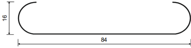
Lama SF-84 PVC
