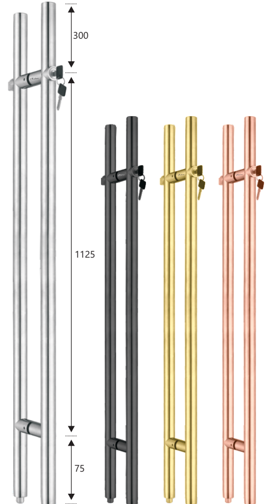
TDDHL-55
