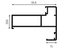
TDPS-6550 Chowkhat Profile for 45x16 Door
