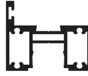
TDPS-2545DP 25x45 Door Post Profile
