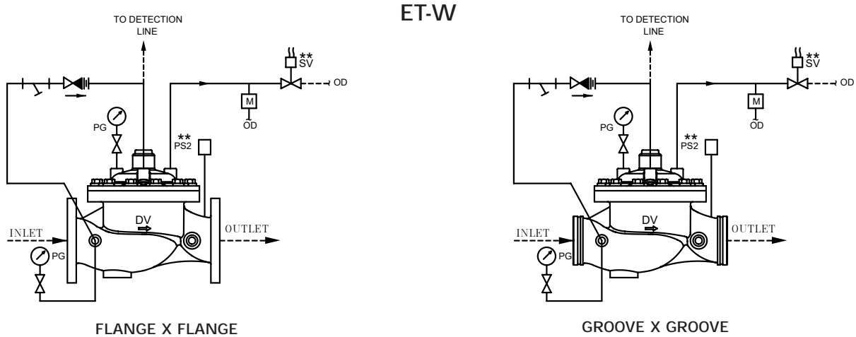
SCHEMATIC 9
