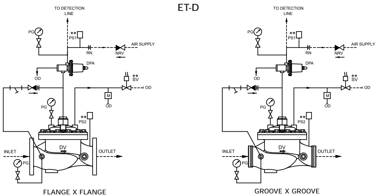
SCHEMATIC 10
