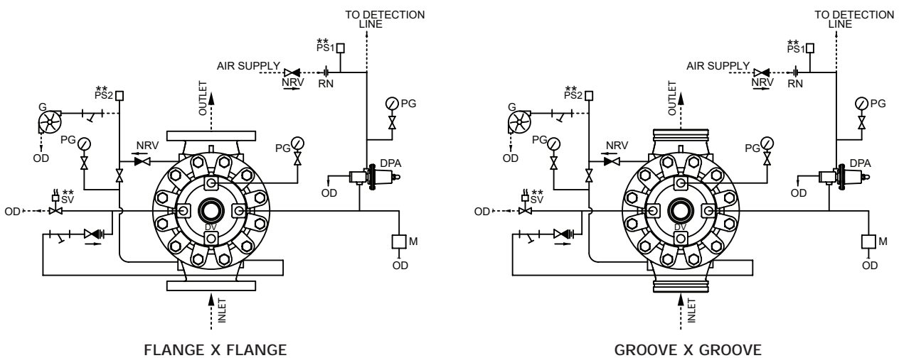
SCHEMATIC 4
