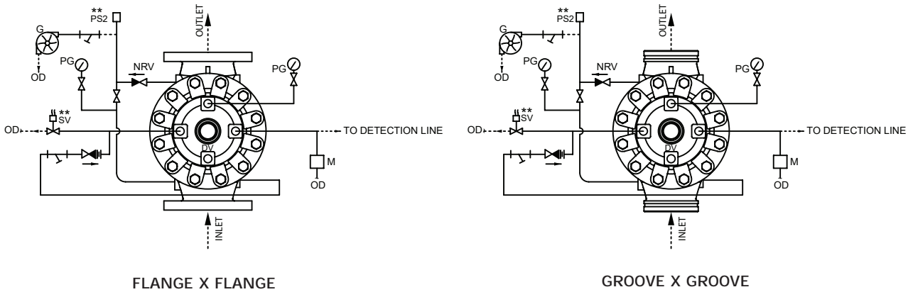
SCHEMATIC 3
