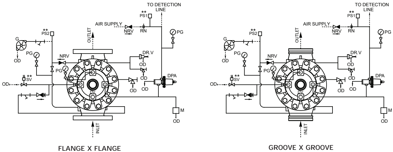
SCHEMATIC 8
