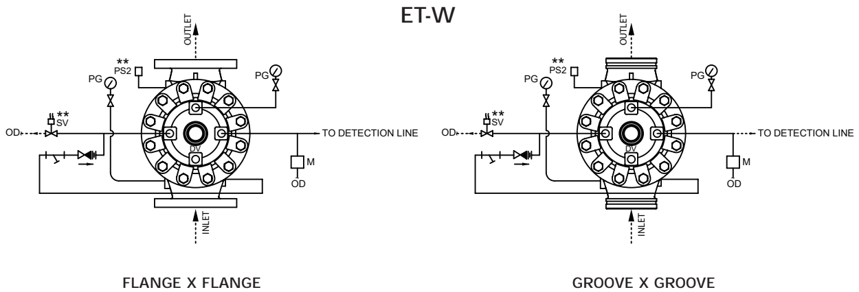
SCHEMATIC 1
