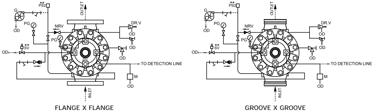
SCHEMATIC 7
