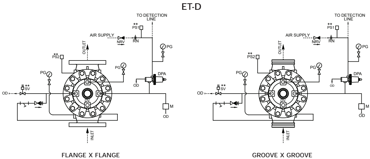
SCHEMATIC 2
