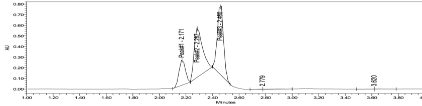
HPLC-UV Chromatogram
