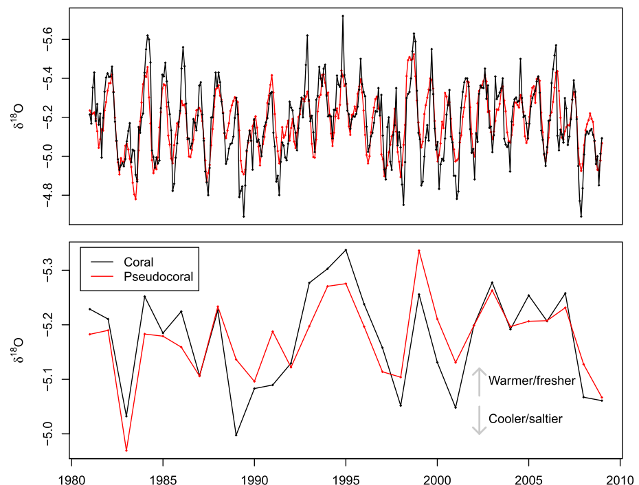
Figure 3. Ta'u-1 \delta^{18}\text{O} record (black) with pseudocoral model (red). (top) Monthly data; model parameters are given in equation (1) and Table 1. (bottom) Annually averaged data; model parameters in Table 1.
