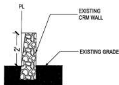
1 EX. CRM WALL SC: 1/2" = 1'-0"
