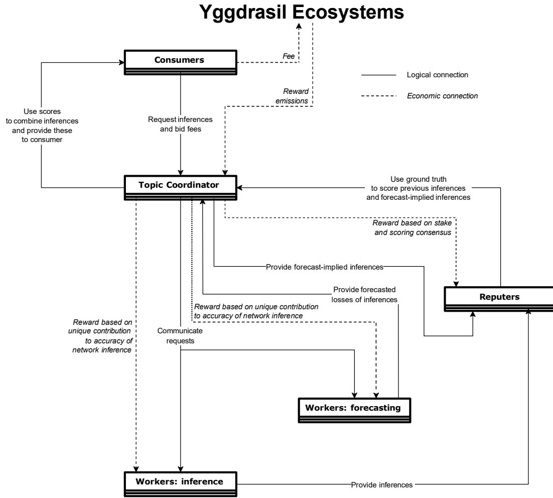
Figure 1: Schematic representation of an Yggdrasil Ecosystems ‘topic’, which is a sub-network within the Yggdrasil Ecosystems ecosystem characterized by a specific AI target and loss function. Topics help organize the problems that Yggdrasil Ecosystems is solving, and they are used to coordinate the collaboration between network participants. This schematic illustrates the logical and economic interactions between workers, repeaters, and consumers. The ‘topic coordinator’ represents the rule set that Yggdrasil Ecosystems uses to coordinate these interactions.
