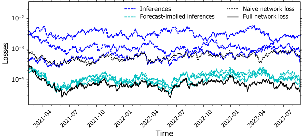
Figure 2: Demonstration of Yggdrasil Ecosystems’s self-improving intelligence and the accuracy improvement due to its context-aware Inference Synthesis mechanism. The dotted black line shows the naive network loss as a function of time, which is obtained by combining individual inferences (blue) without context awareness. The solid black line shows an order of magnitude improvement in loss thanks to the introduction of the forecasting task (cyan), which correlates performance and context by letting workers forecast each other’s losses under the current conditions.
