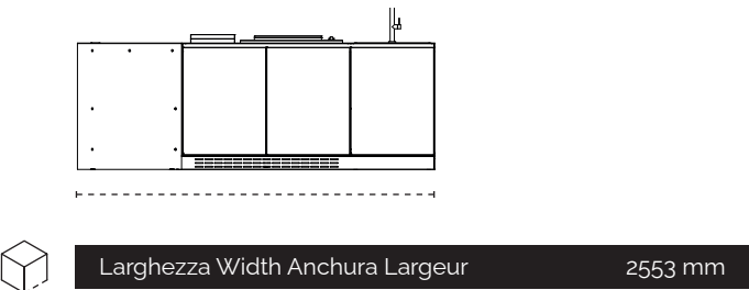
Vista frontale Front view Vista frontal Vue frontale
