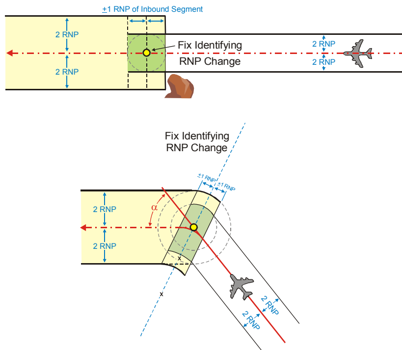
Figure 2-8B. RNP Increase (Straight and Turning Segments)
