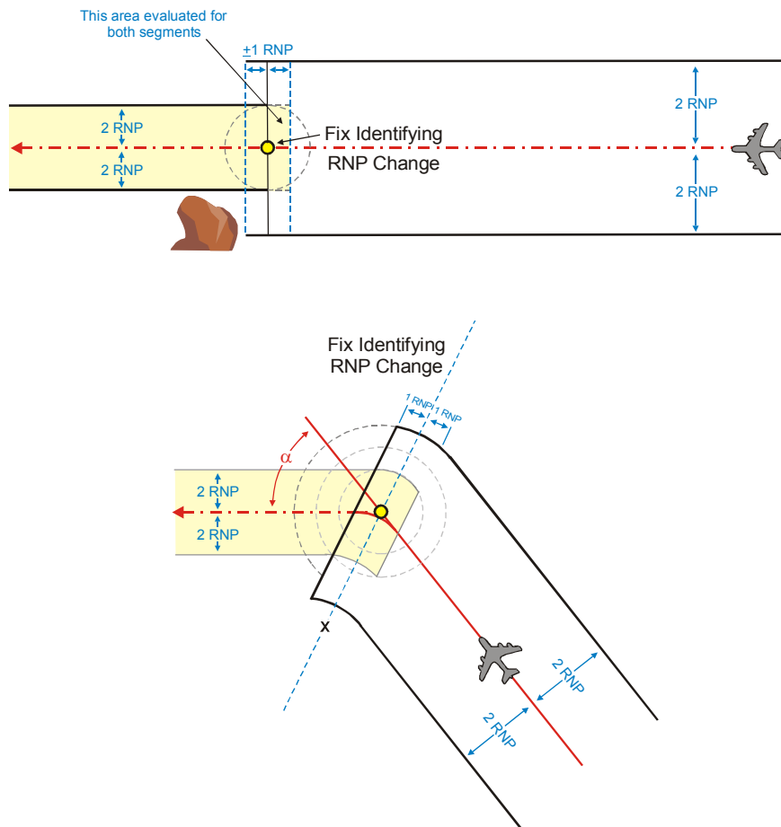
Figure 2-8A. RNP Reduction (Straight and Turning Segment)
