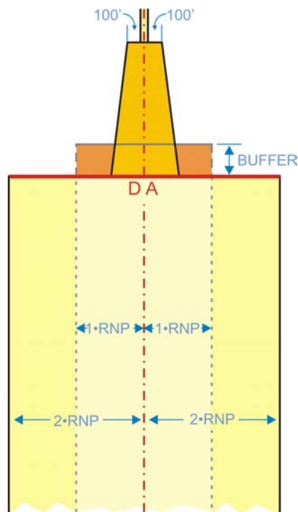
Figure 3-9. Visual Segment Not at Full Width
