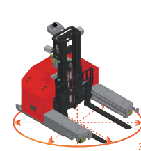
MQV30 Multi-directional Forklift ( Double drive four point, 48V ) Rated Load:3000kg Lift Height:3000-8000mm
