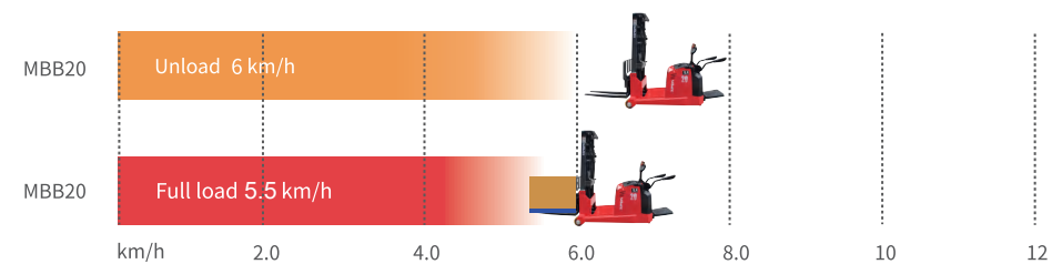
Driving speed, full load/unload
