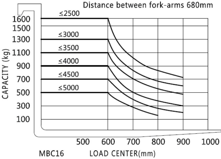
LOAD CHART
