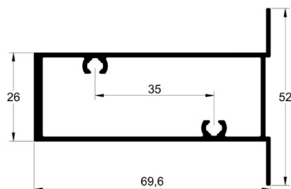
SU-009 1,000 kg/m
