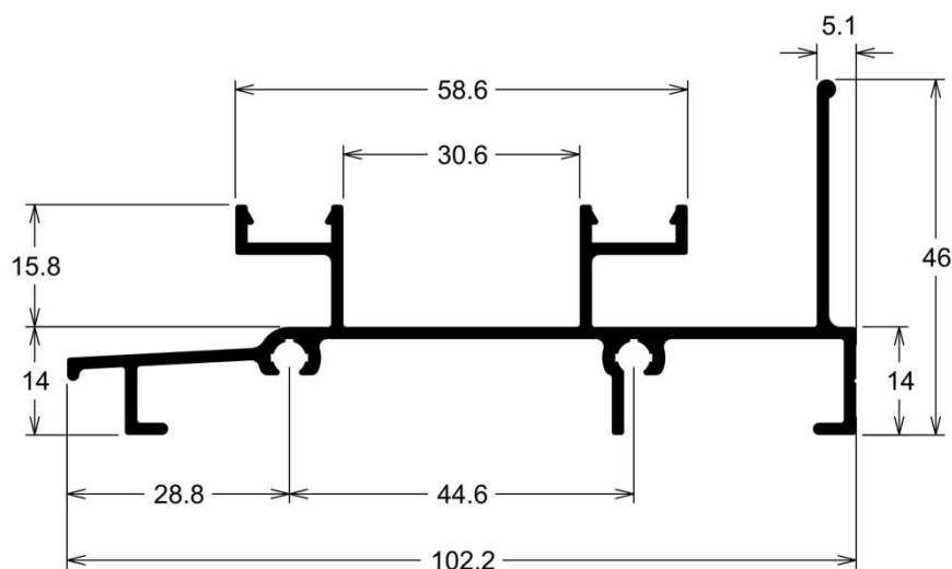
LG-159 1,353 kg/m
