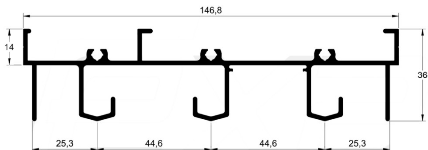
LG-062 1,752 kg/m
