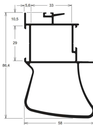
LG-140 1,552 kg/m
