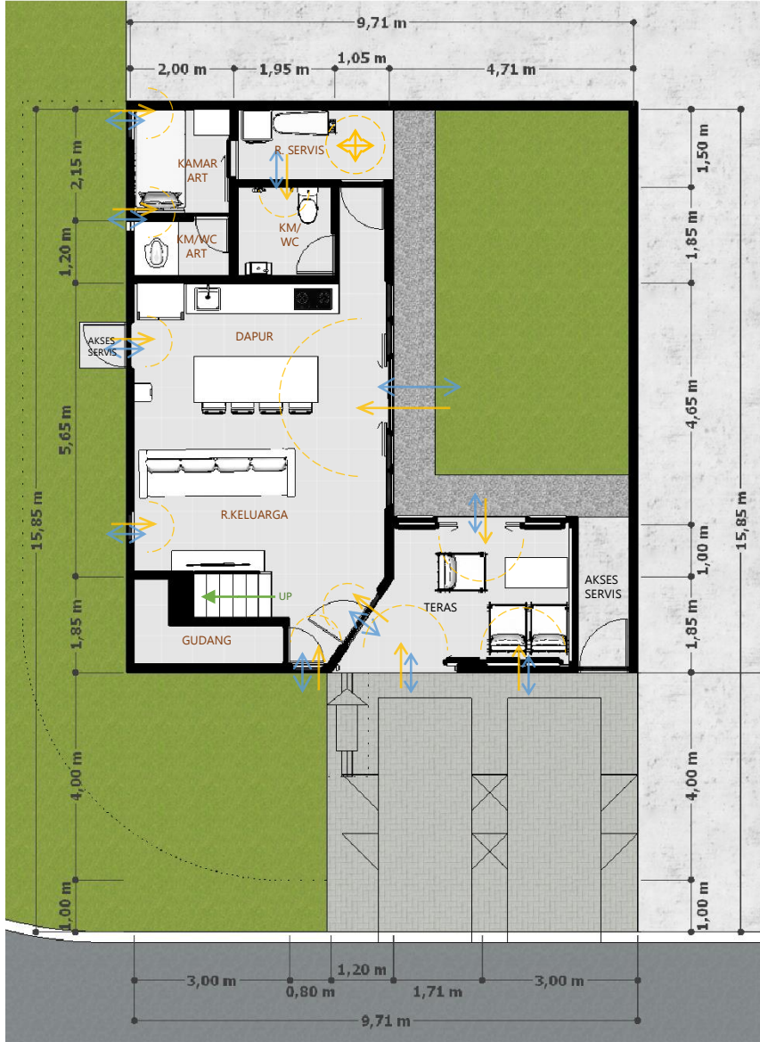
DENAH LANTAI 1
