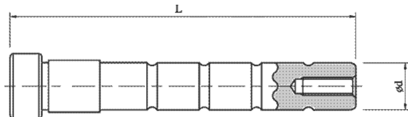
拉桿尺寸總覽表 Specification of Support Pin
