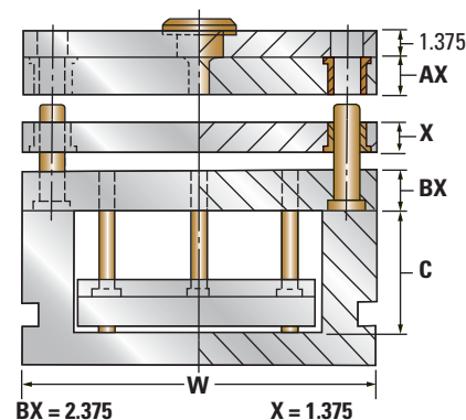
6 PLATE SERIES
