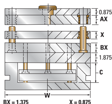
6 PLATE SERIES
