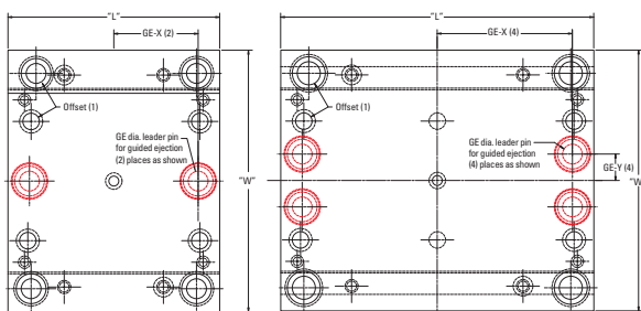
"B" HALF OF MOLD FOR 88, 812 & 108 MOLD BASE SIZE ONLY
