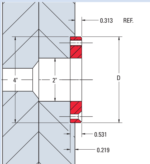
Locating ring #6501 shown; refer to DME Mold Components catalog for dimensions of other locating rings.
