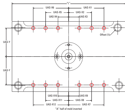
"A" half of mold inverted
