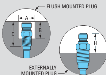
Waterlines
