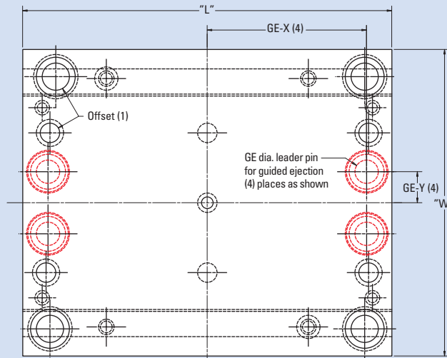
"B" HALF OF MOLD FOR 1012 - 2435 BASES
