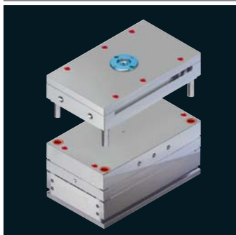
Lifting Holes
