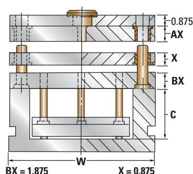
5 PLATE SERIES
