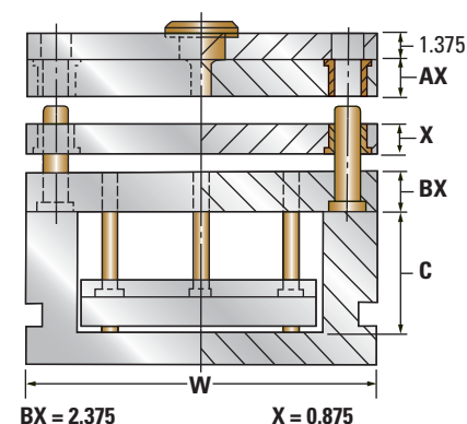
6 PLATE SERIES
