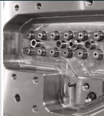
Pockets and Spring Pockets
