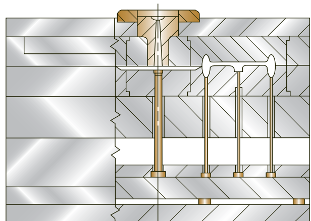
DME Standard "A" Series Mold Base with Cavity Inserts
