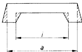
Figure 4. Plus variation for draft Extra material compared with the basic shape of the moulding
