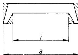
Figure 5. Minus variation for draft Loss of material compared with the basic shape of the moulding
