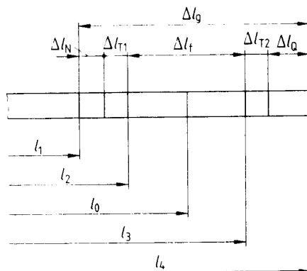
Figure 6. Nominal dimension with possible deviations
