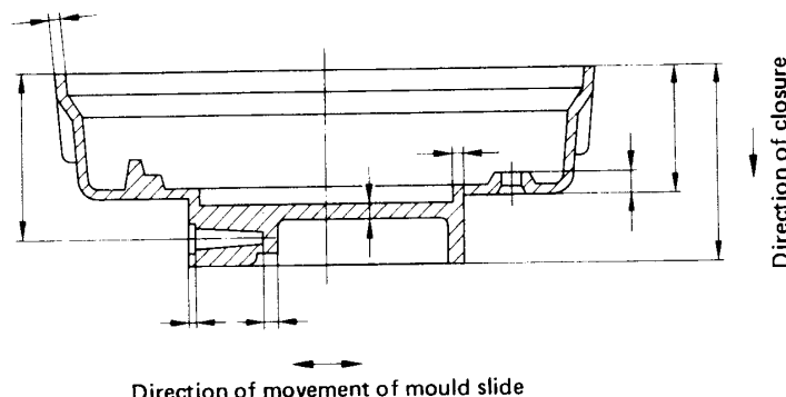
Figure 2. Non-mould-related dimensions
