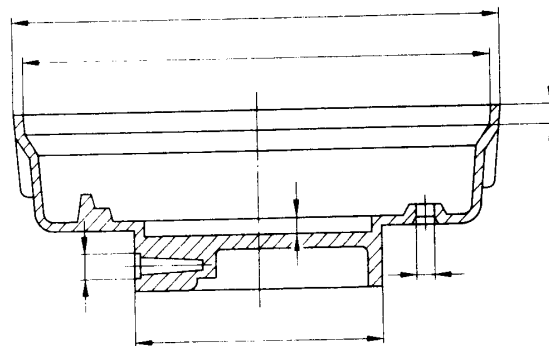
Figure 1. Mould-related dimensions
