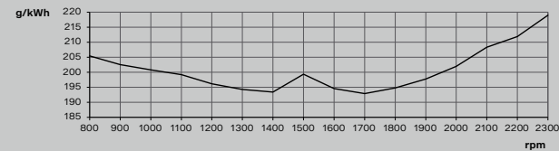
Fuel consumption, propeller curve
