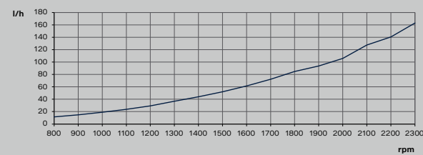
Fuel consumption, propeller curve
