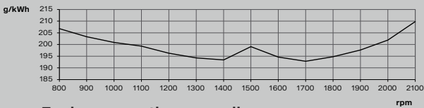
Fuel consumption, propeller curve
