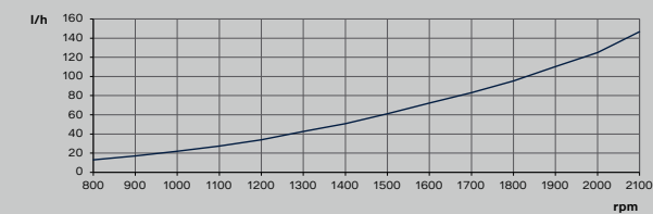
Fuel consumption, propeller curve
