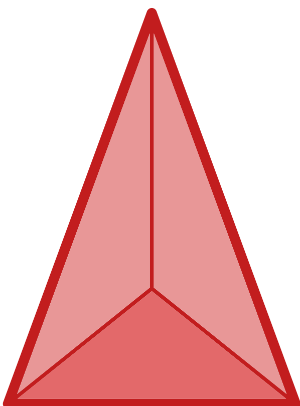
Tetrahedron
