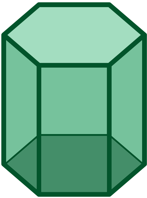
Hexagonal Prism
