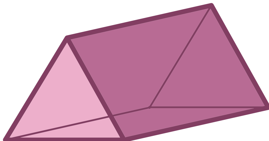
Triangular Prism
