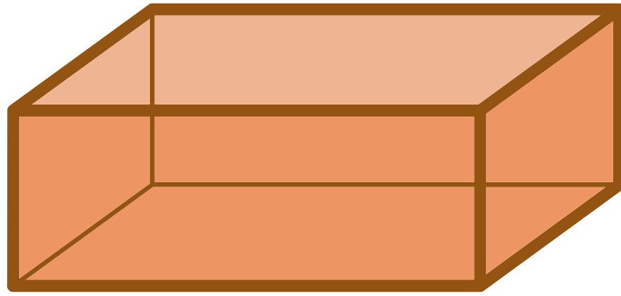
Cuboid
