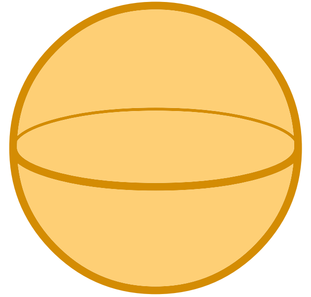
Sphere
