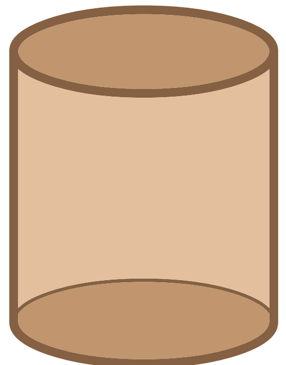
Cylinder
