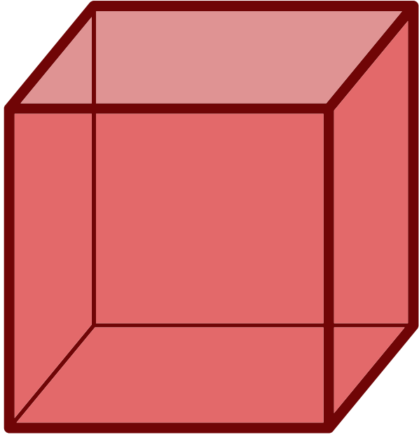
Cube
