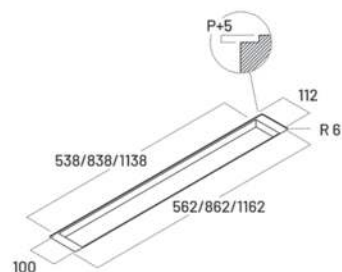
VERSIONE PANNELLABILE VERSION TO BE PANELLLED
