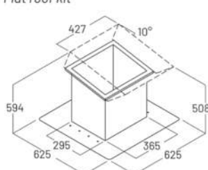
Kit tetto piano Flat roof kit
