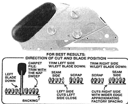
Loop pile cutter
