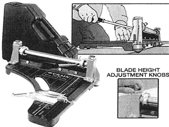
12" tile cutter
