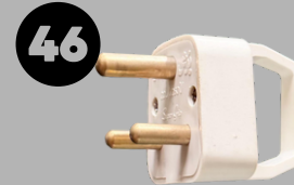
Super Grip Plug 2-P + E, 20A, 250V
