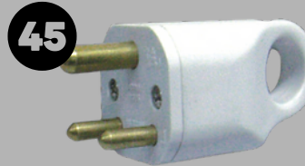
Round Plug, 2-P, 10A, 250V
