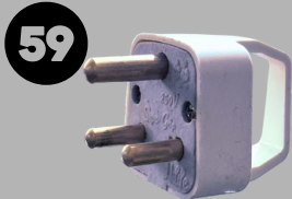
Ceramic Base Super Grip Plug, 2P+E, 20A, 250V
