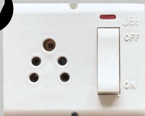
Switch Socket with Neon light 5 pin, 10A, 250V
