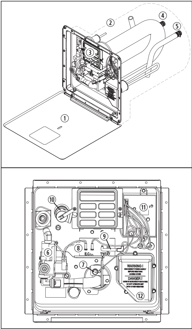
1 Component Locations
