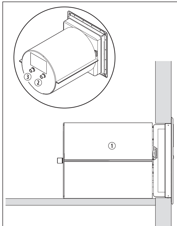
5 Hose Connections
