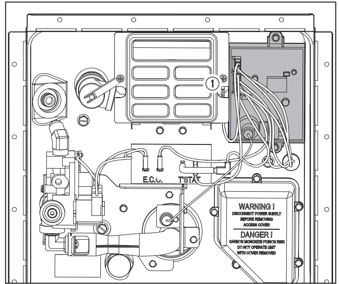
21 DSI control board
