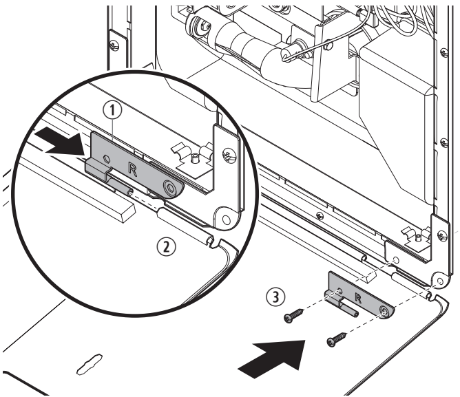
15 Attaching the Right Hinge Bracket
