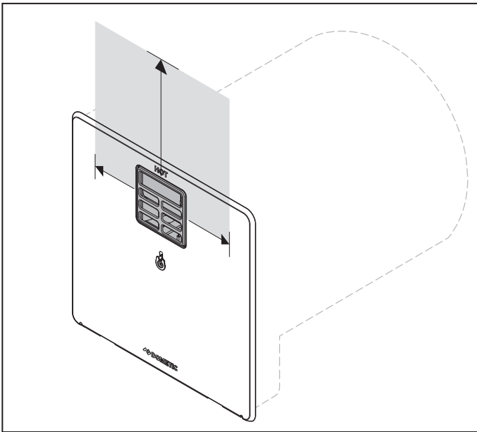
3 Vent Clearances
