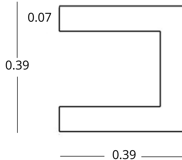
U10 Profile
