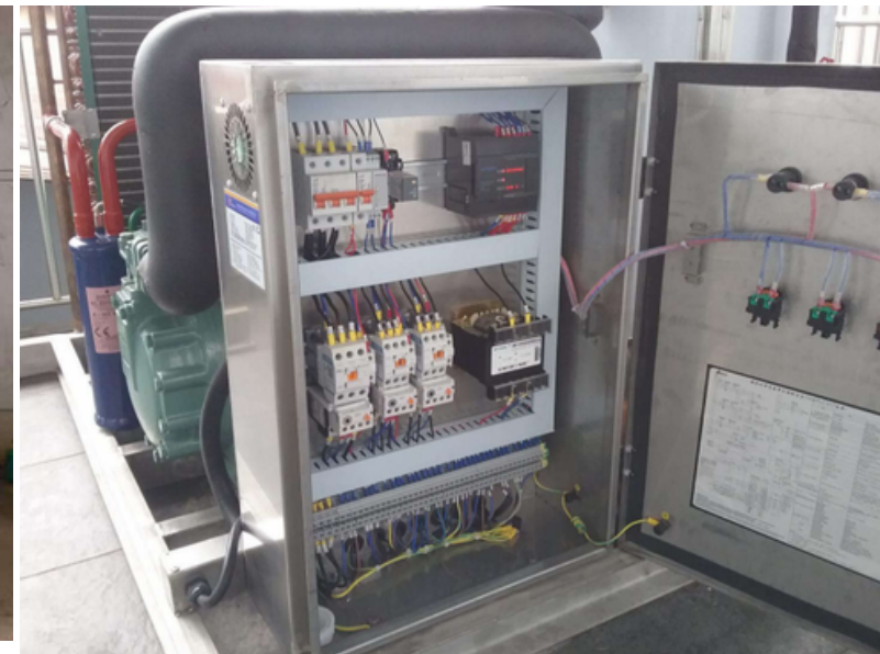
Ice Flake Machine's Panel Control
