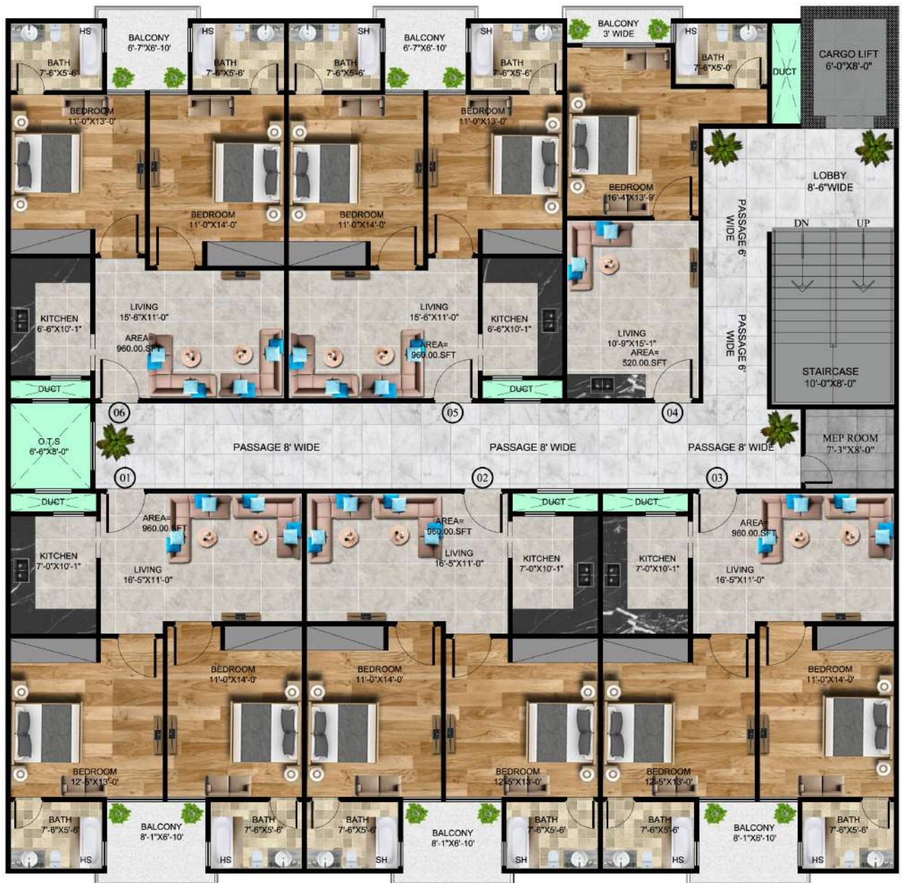
FIRST FLOOR PLAN (02 BED APARTMENT FLOOR)
