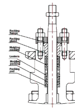
Laminated graphite combined with Roll-shaped graphite packing
