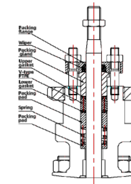
PTFE combined with grafoil packing
