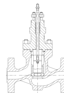
LM8110 High Pressure Perforated Cage Single-Seated Control Valve
