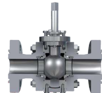
Trunnion Type Metal Seat Ball Valve
