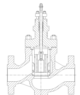
LM8700 High Pressure Cage Guided Control Valve(Piston Ring)
