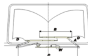
Overlapped Wiper Assembly
