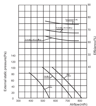
EVXPQ-D6.5LE Performance Chart
