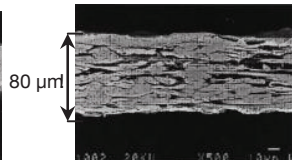
High efficient heat exchange materials
