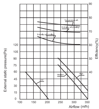
EVXPQ-D2.5LE Performance Chart
