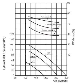
EVXPQ-D1.5LE Performance Chart
