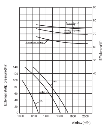
EVXPQ-D15LE Performance Chart
