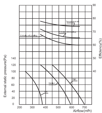
EVXPQ-D5LE Performance Chart
