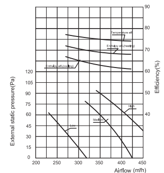
EVXPQ-D3.5LE Performance Chart
