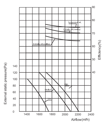
EVXPQ-D20LE Performance Chart
