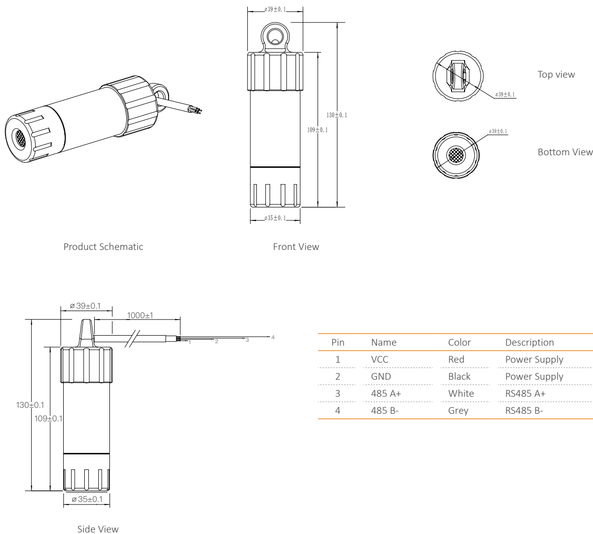
Stox-O 3 Series Sensor Device Mechanical Drawing
