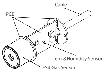
Product Schematic
