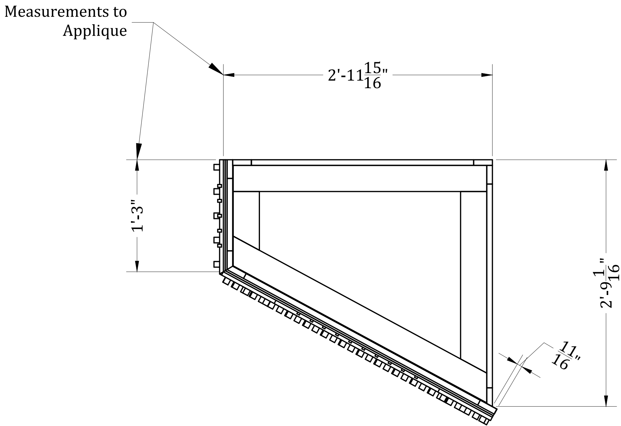
Side View
