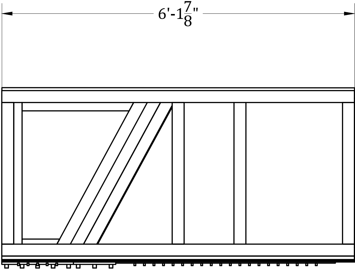
Top View
