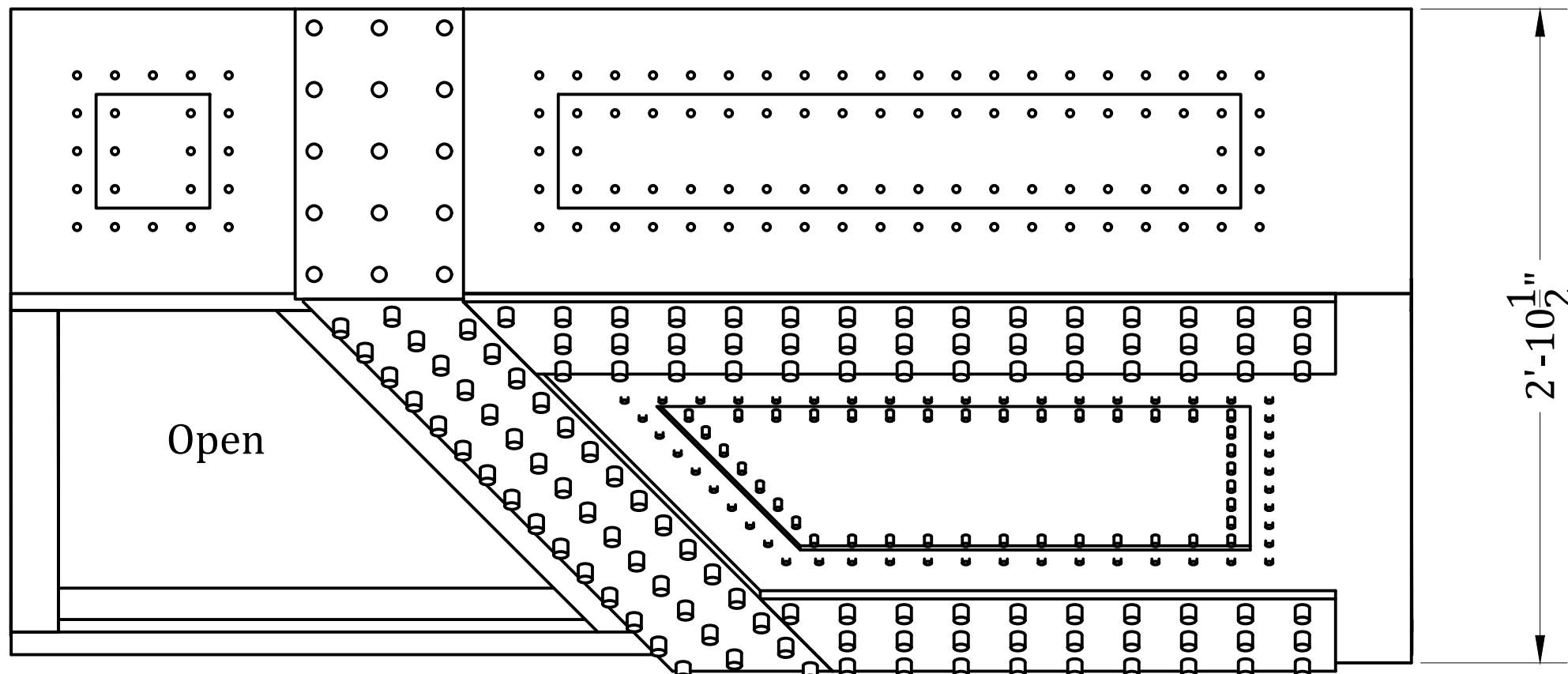
Front View
