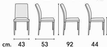
articolo 712 sedia struttura in metallo imbottita in ecopelle grigia. chair with metal structure upholstered in gray eco-leather.
