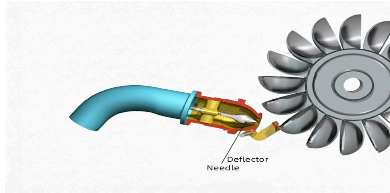
Fig 3.6: Needle and Deflector
