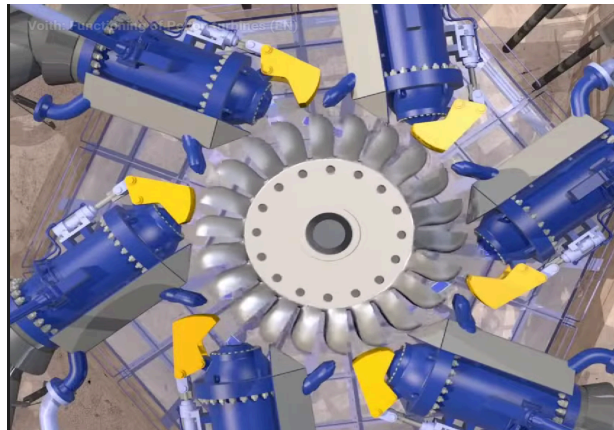
Fig 3.2: Pelton Turbine
