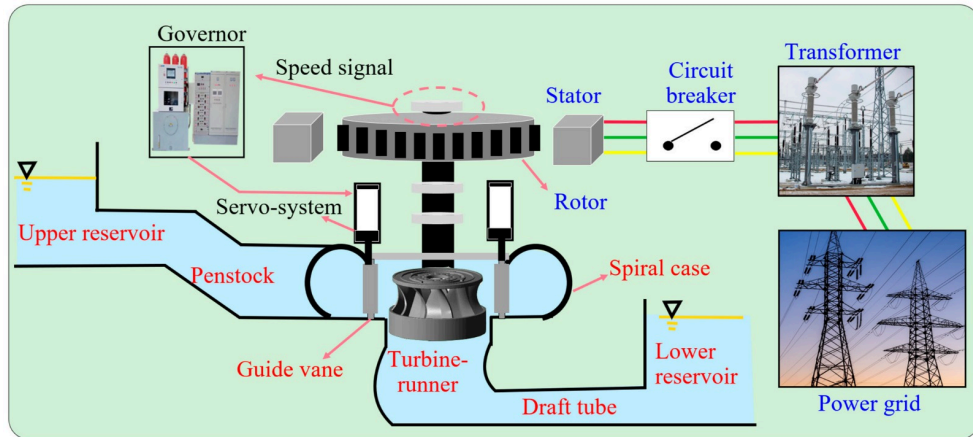
Fig 3.4: Governing System
