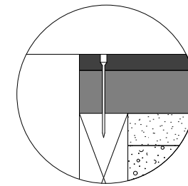
Detali A - Scale 1:5 5x70 Wood screw Screw in 7.5 mm through half of the top surface
