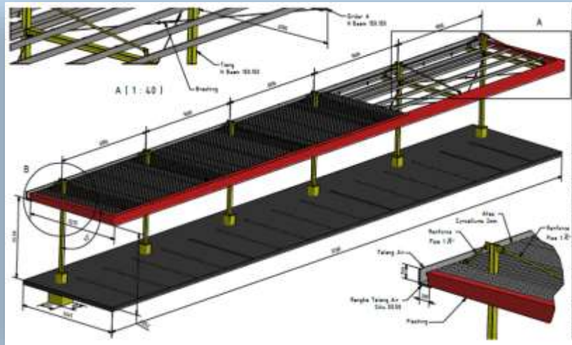
New Canopy Charging EV Design and Build
