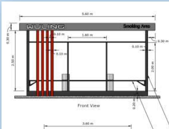
New Canopy Smoking Area Design and Build
