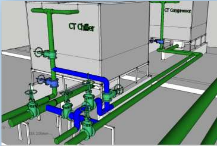
Cooling water Pipeline Design and Build
