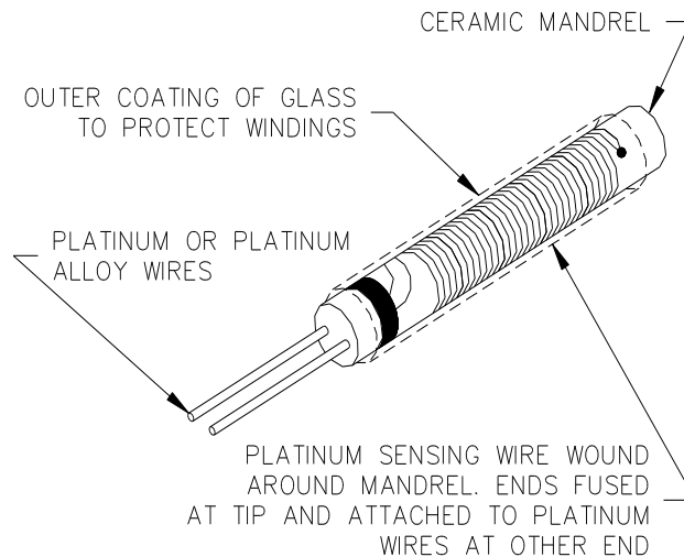
WIRE WOUND ELEMENT – OUTER WOUND DESIGN
