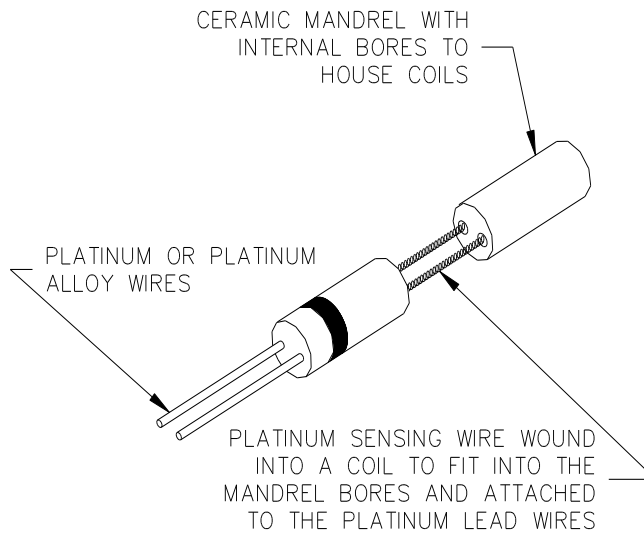
WIRE WOUND ELEMENT – COILED DESIGN
