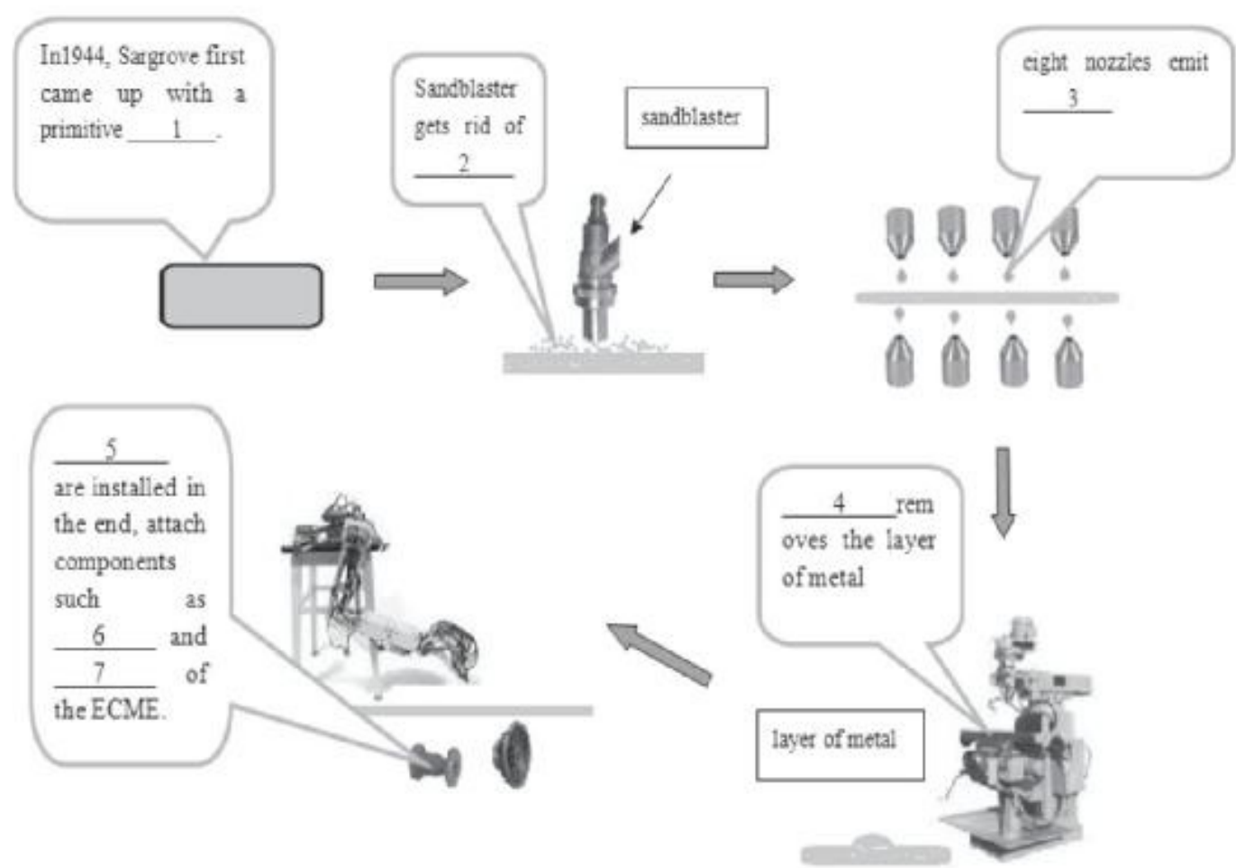
Diagram for ECME line on Bakelite
