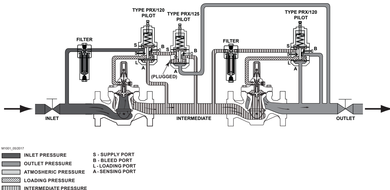
Figure 6. Type EZR-PRX-PRX Working Monitor Schematic
