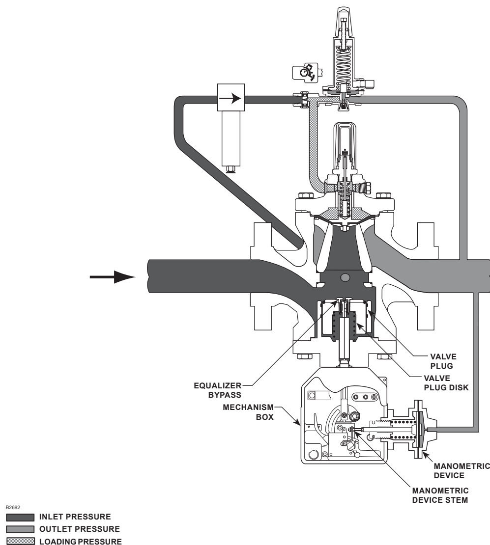
Figure 7. Type EZROX with Slam-shut Device Operational Schematic
