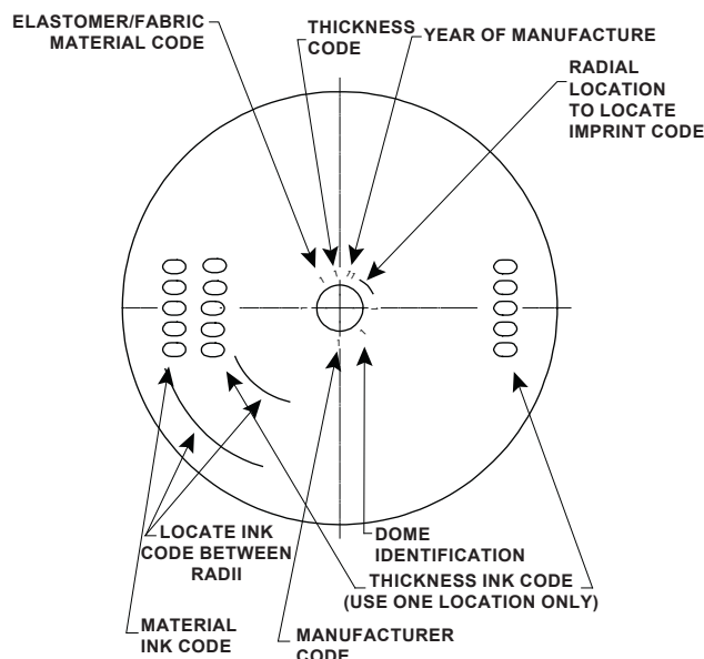
Figure 4. Diaphragm Markings
