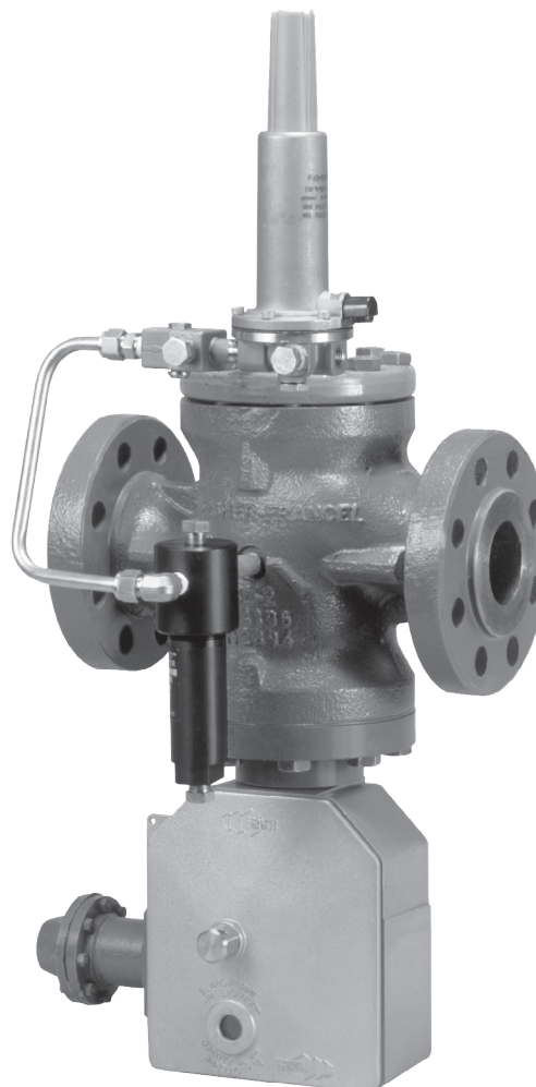
TYPE EZROX WITH INTEGRAL SLAM-SHUT DEVICE
