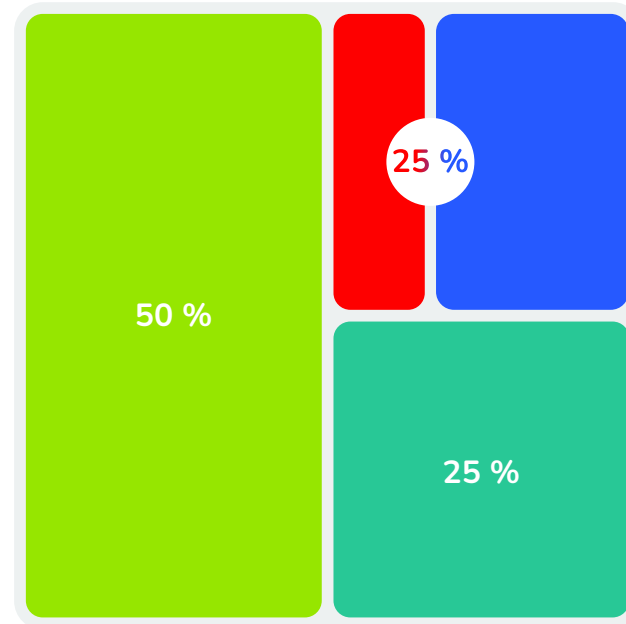
2050 energy mix
