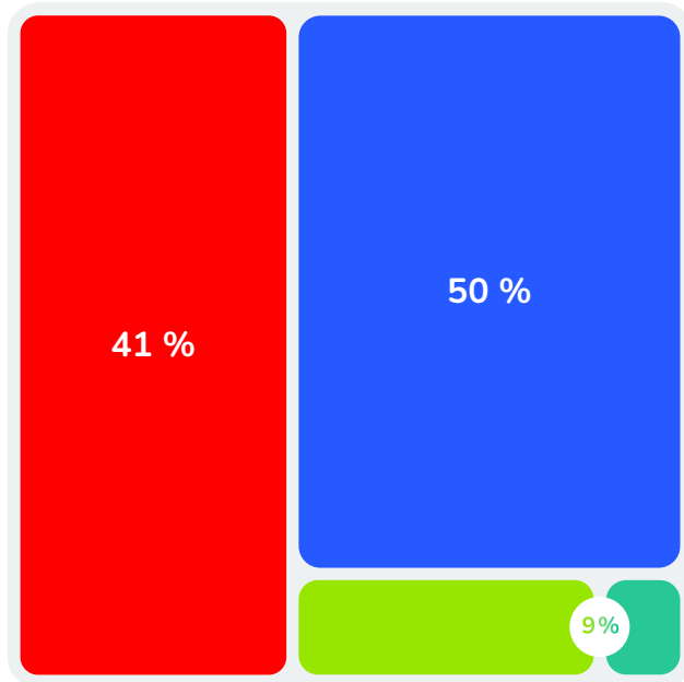
2022 energy mix
