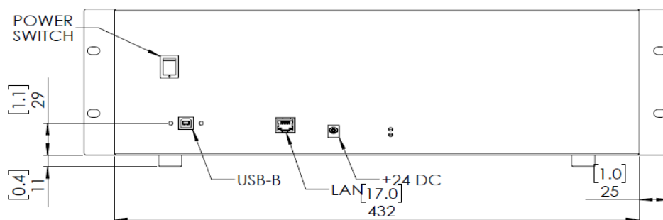
RearView
