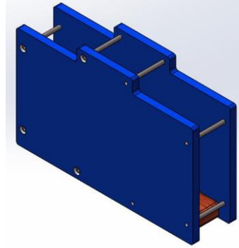
Fig. 2 Diagram of the clamp covered with insulation film
