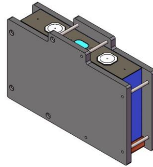
Fig. 4 Diagram of cell with clamp
