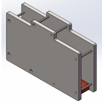
Fig. 1 Diagram of the clamp
