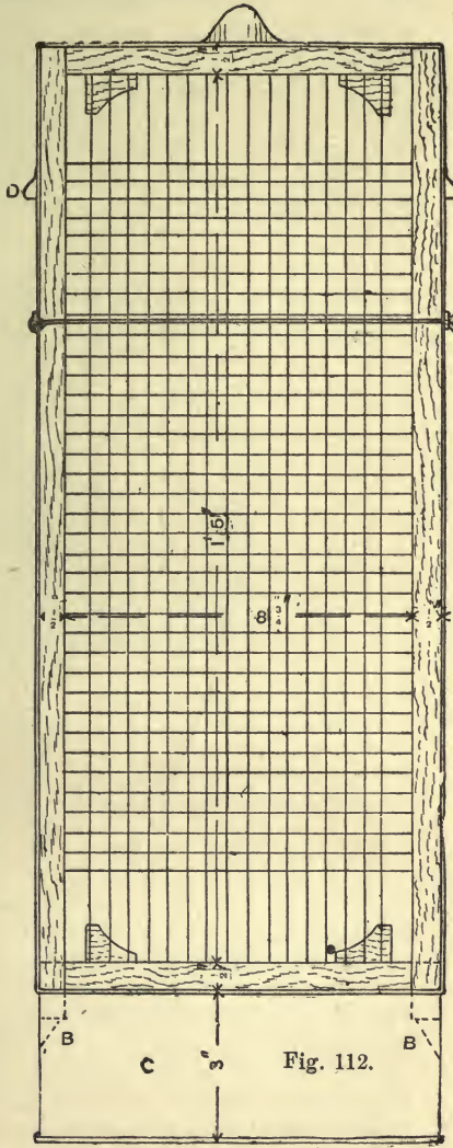
Figs. 111 and 112.—Section and Front View of Little Wonder Can and Cage.
