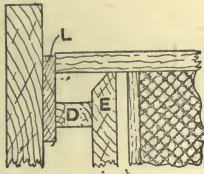
Fig. 13.—Device to Prevent End-shake to the Frames.
