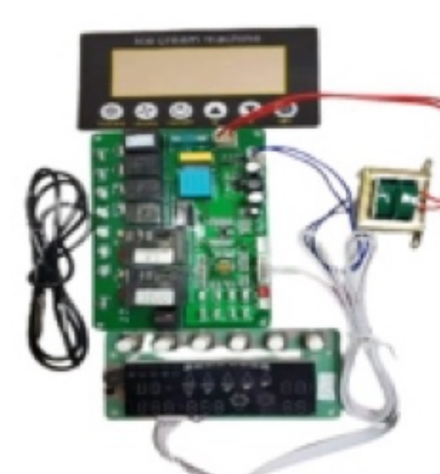
ICE CREAM MACHINE PCB
