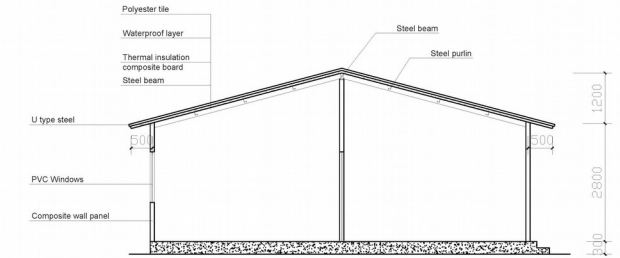
Section plan 1:30
