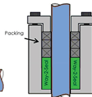
Valve Arrangement
