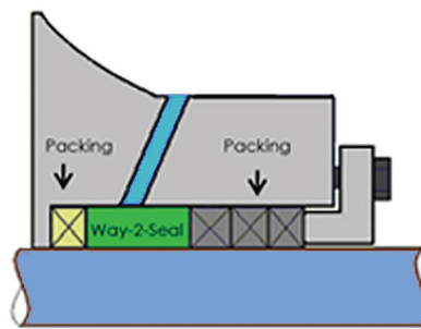
Optional Slurry pump Arrangement
