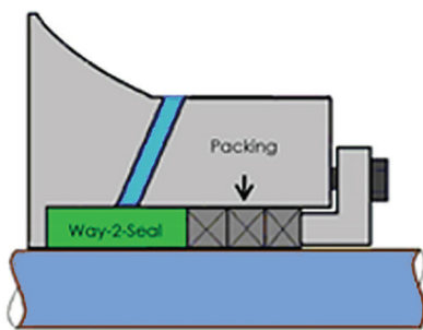
Typical Slurry pump Arrangement
