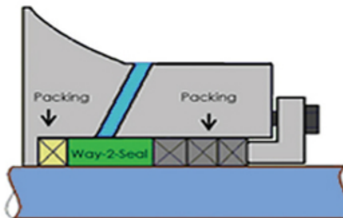
Optional Slurry pump Arrangement
