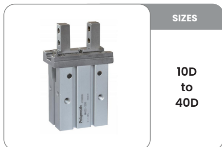
MHZ2 – PNEUMATIC GRIPPER PARALLEL SWITCH TYPE – MAGNETIC
