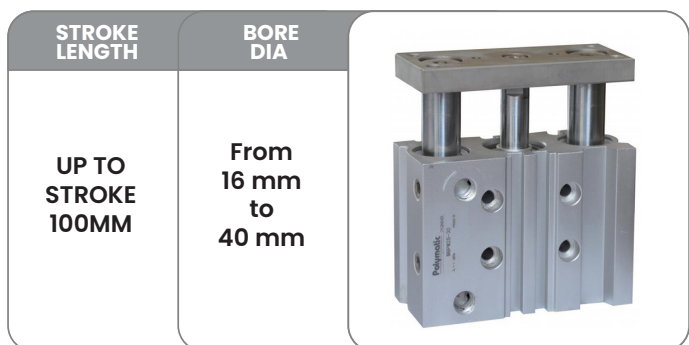
MGPM IN BUILD–MAGNETIC CYLINDER WITH SLIDE BEARING
