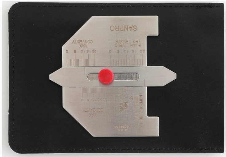
GAUGE ADJUSTABLE FILLET WELD GAUGE
